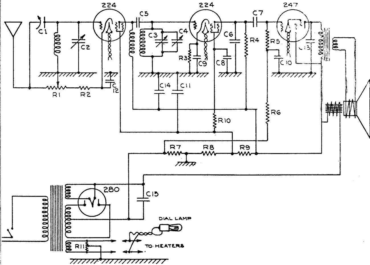
Schematic Wiring Diagram - Model 4 Receiver
